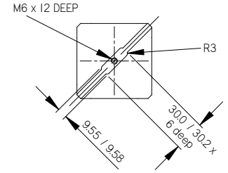
Vane Slot detail both ends
