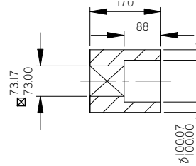
Standard Coupling (supplied with actuator weight 34 lbs/15.4 kg)
