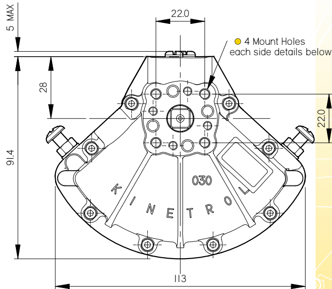
2 Air ports staggered thread details below
