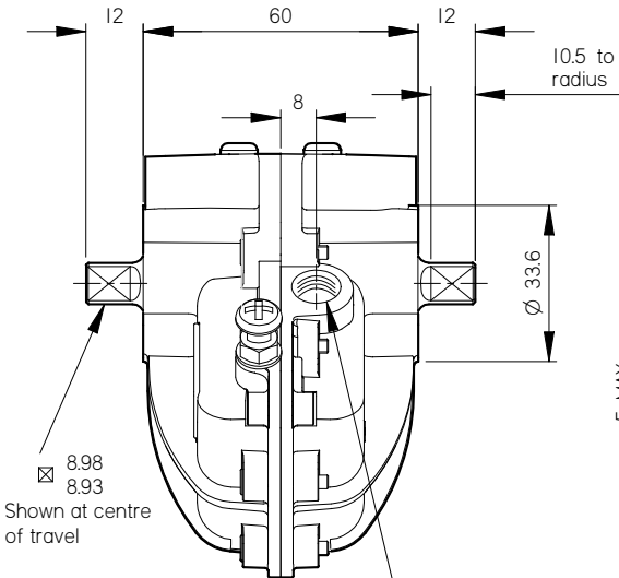
2 Air ports staggered thread details below
