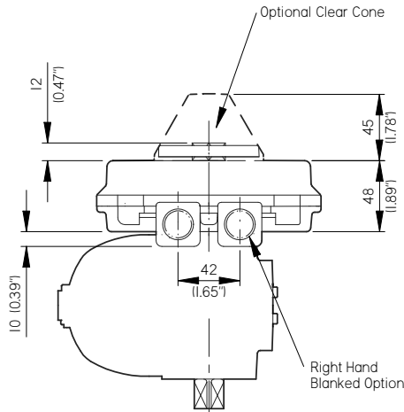
Direct Mount Option
