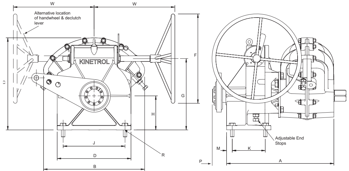
Principal Dimensions mm
