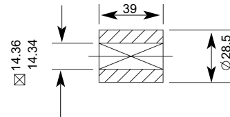
Standard Coupling (supplied with actuator weight 0.31 lbs/0.14 kg)
