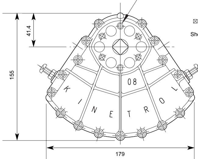
6 Mount holes each side details below
