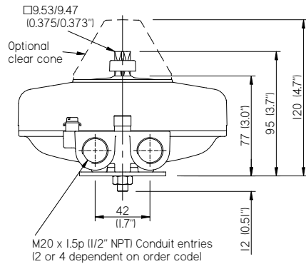
Kinetrol Close Mount Option
