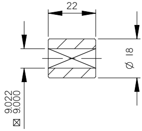
Standard Coupling (supplied with actuator weight 0.07 lbs/0.03 kg)
