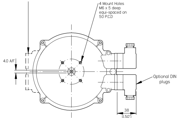
Kinetrol & Namur Discrete Mount Option
